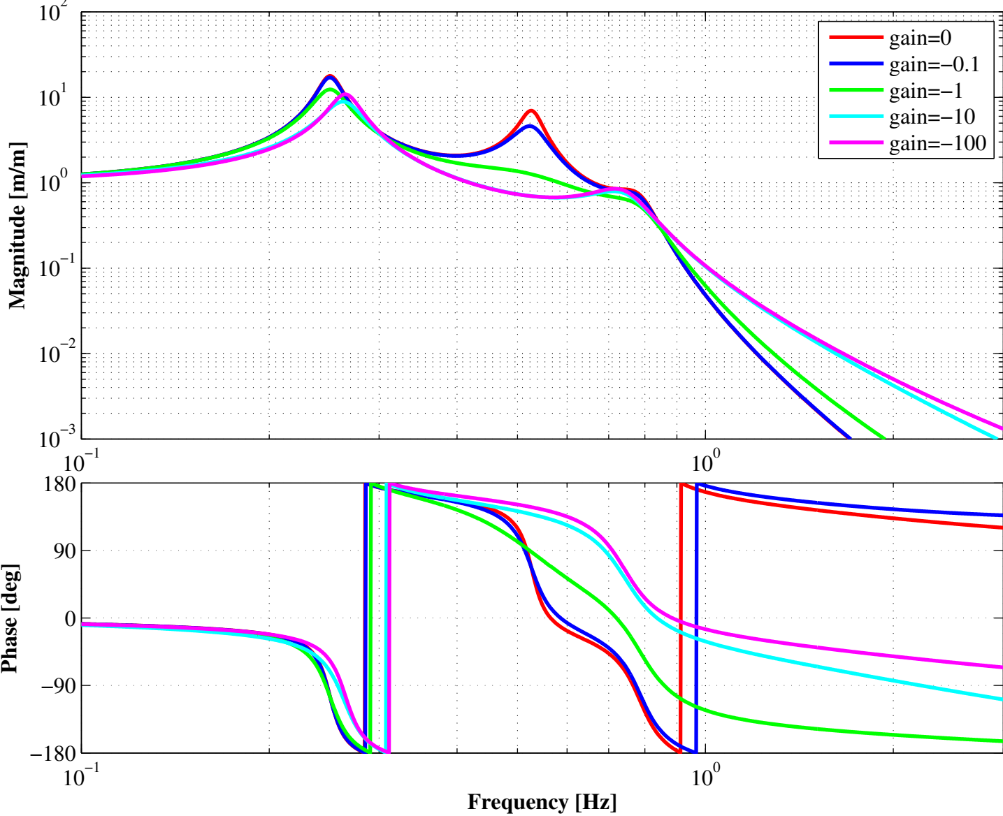
Transfer function from VGND to VTM with IM-OSEM damping
