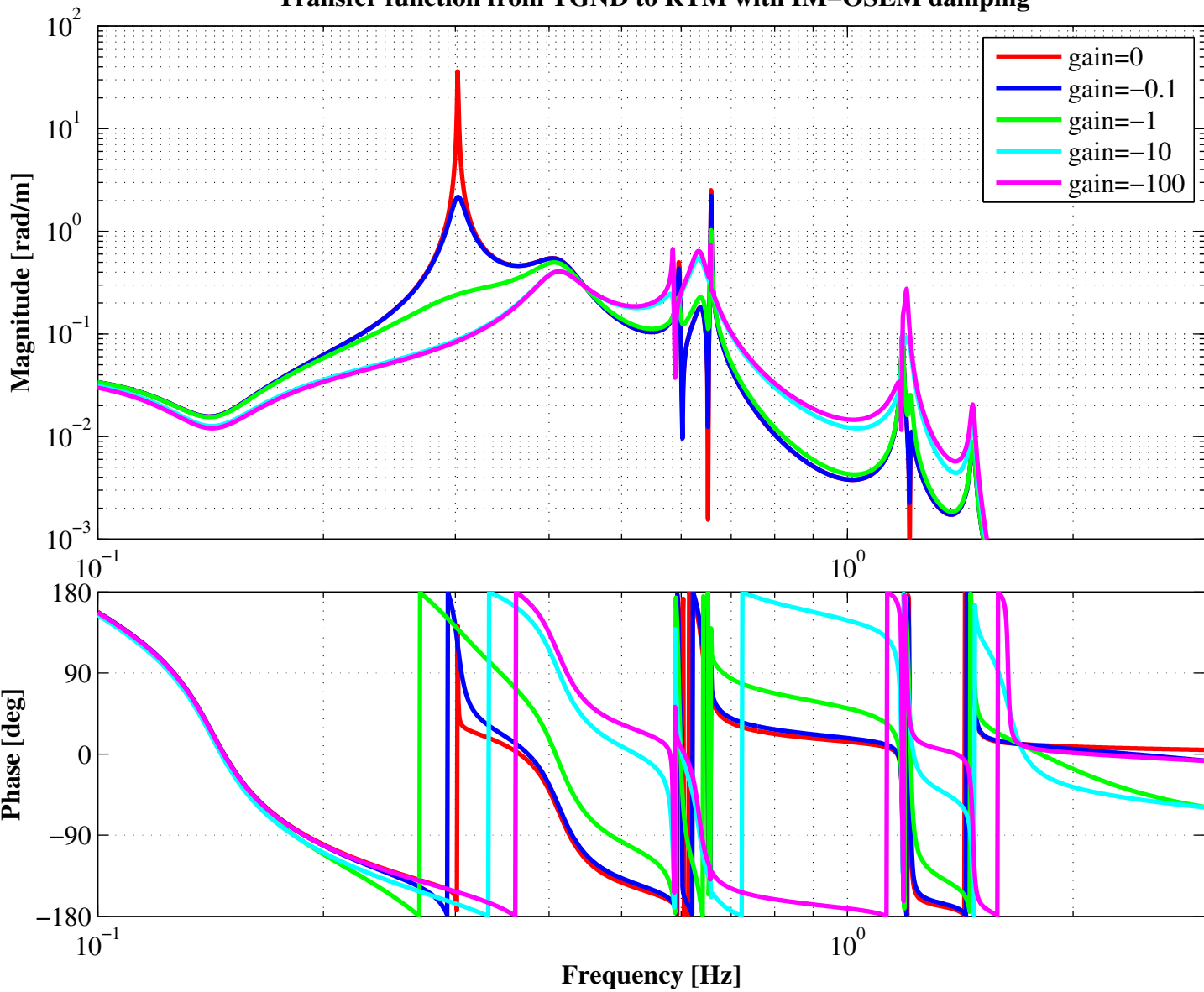
Transfer function from TGND to RTM with IM-OSEM damping
