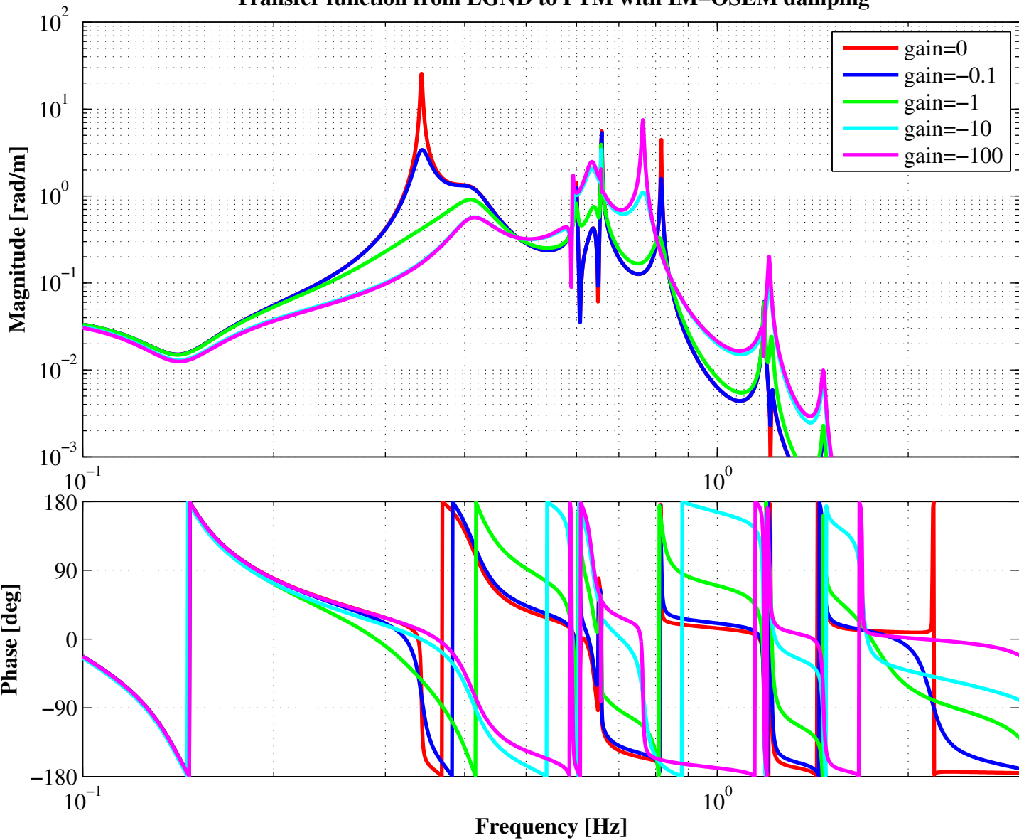
Transfer function from LGND to PTM with IM-OSEM damping
