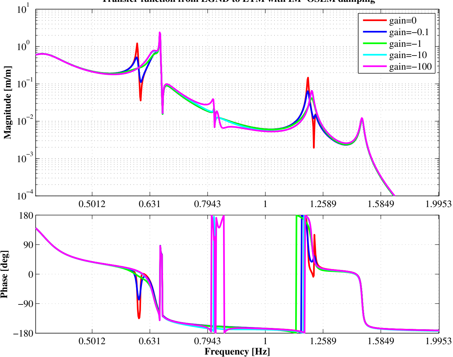
Transfer function from LGND to LTM with IM-OSEM damping
