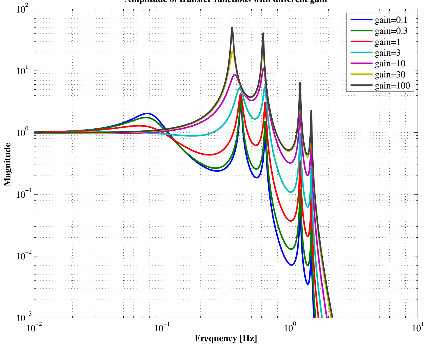
Amplitude of transfer functions with different gain
