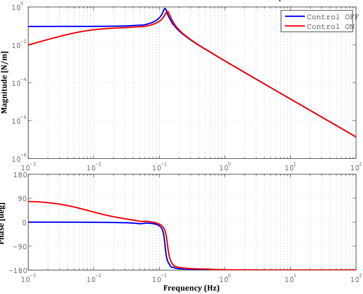
Transfer Function Bode Plot from actYIP to LVDT y_{IP}
