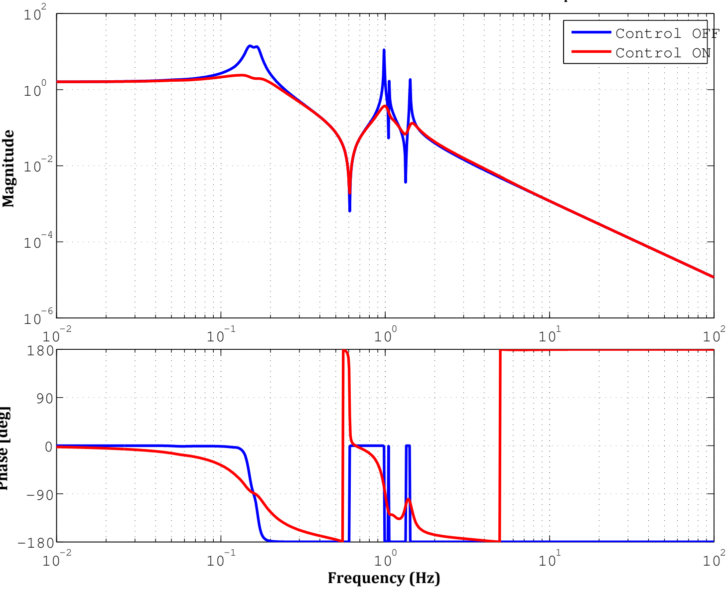
Transfer Function Bode Plot from actYIM to OSEM \gamma_{IM}
