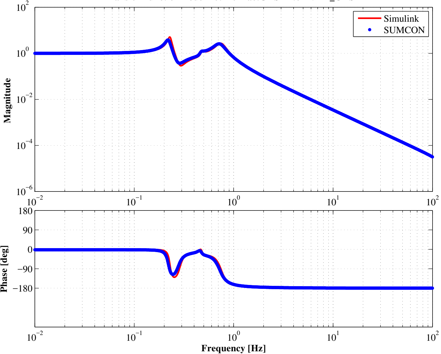
Transfer Function Bode Plot from actGASF1 to LVDT_GASF1
