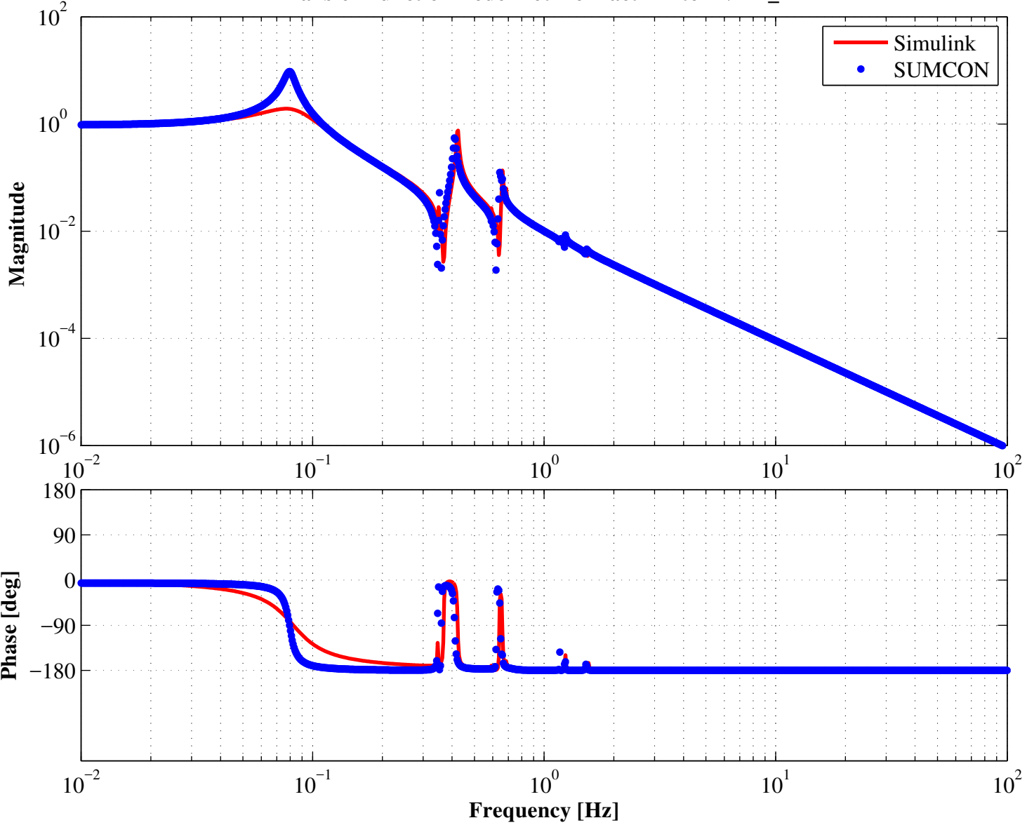
Transfer Function Bode Plot from actLIP to LVDT_LIP
