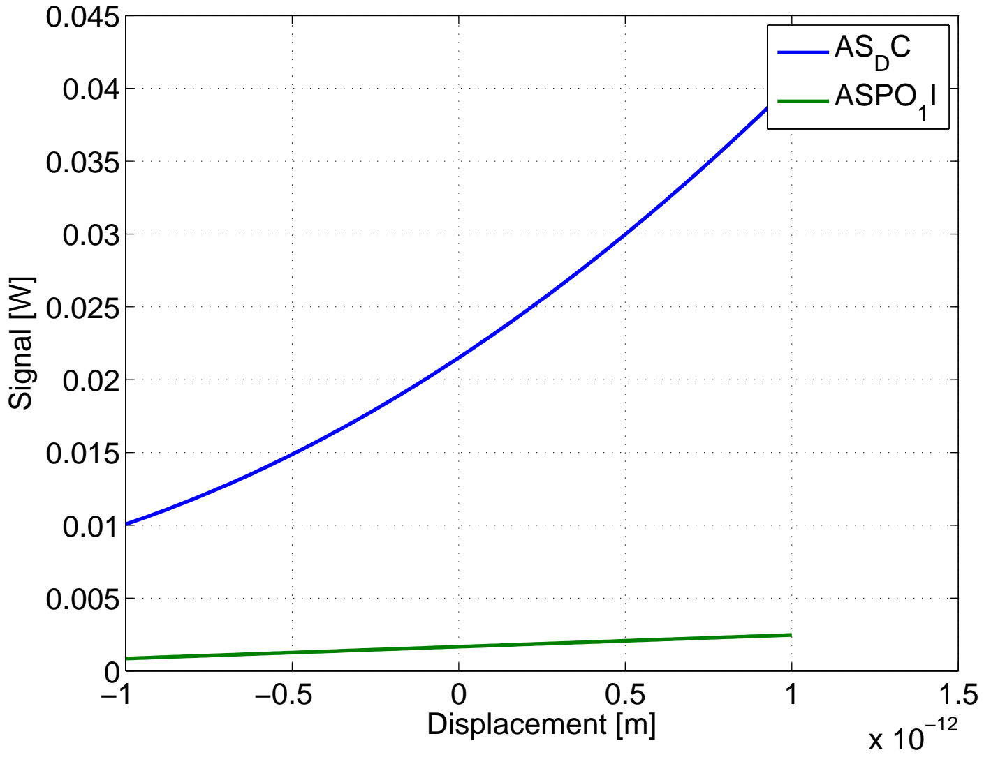
DARM Sweep
