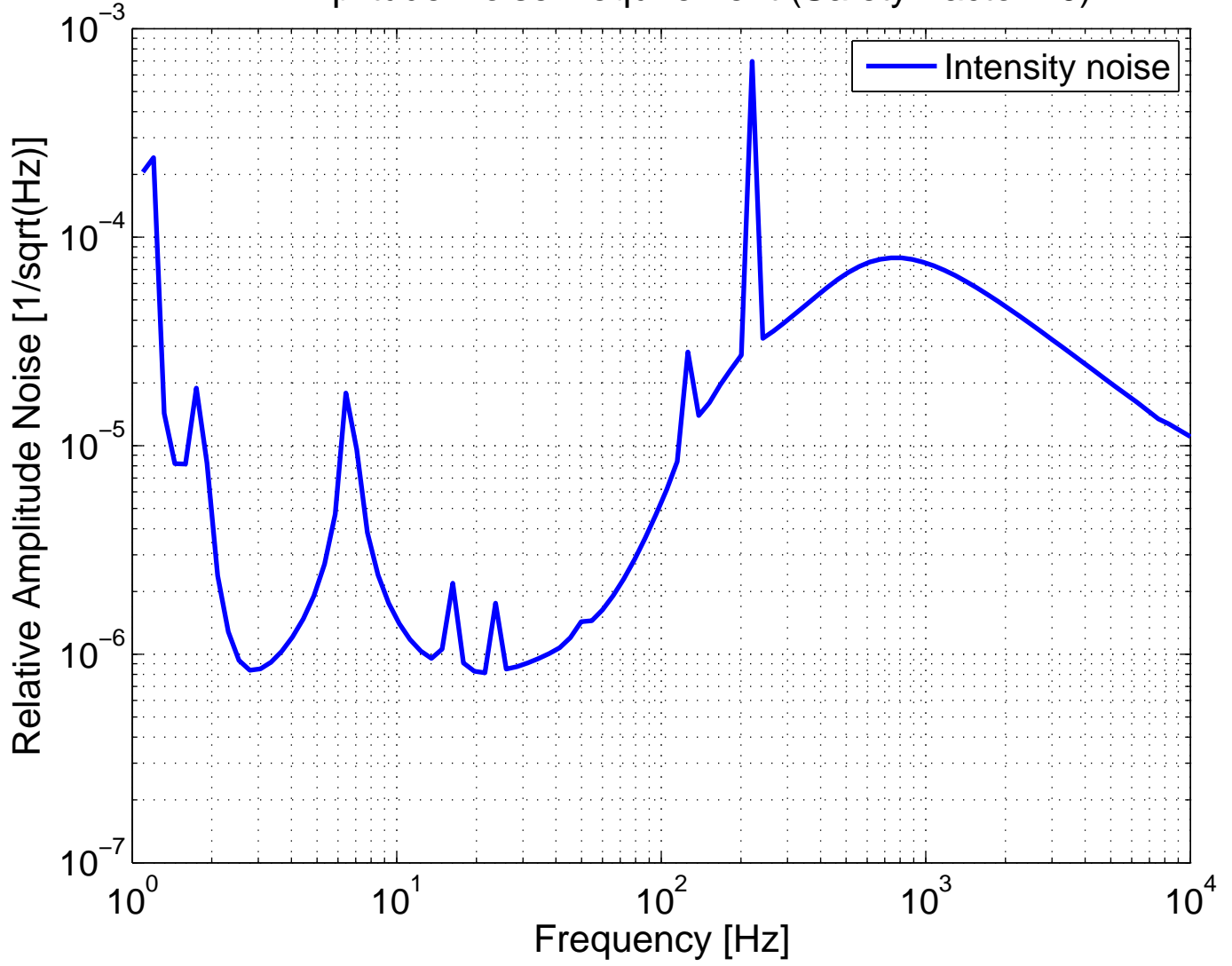
f2 Amplitude Noise Requirement (Safety Factor 10)
