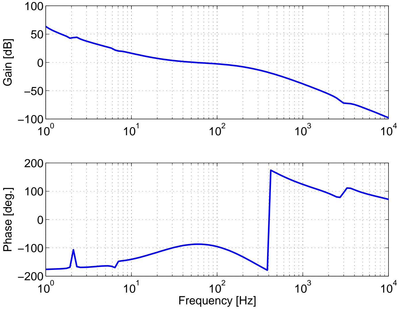
PRC Open Loop Gain
