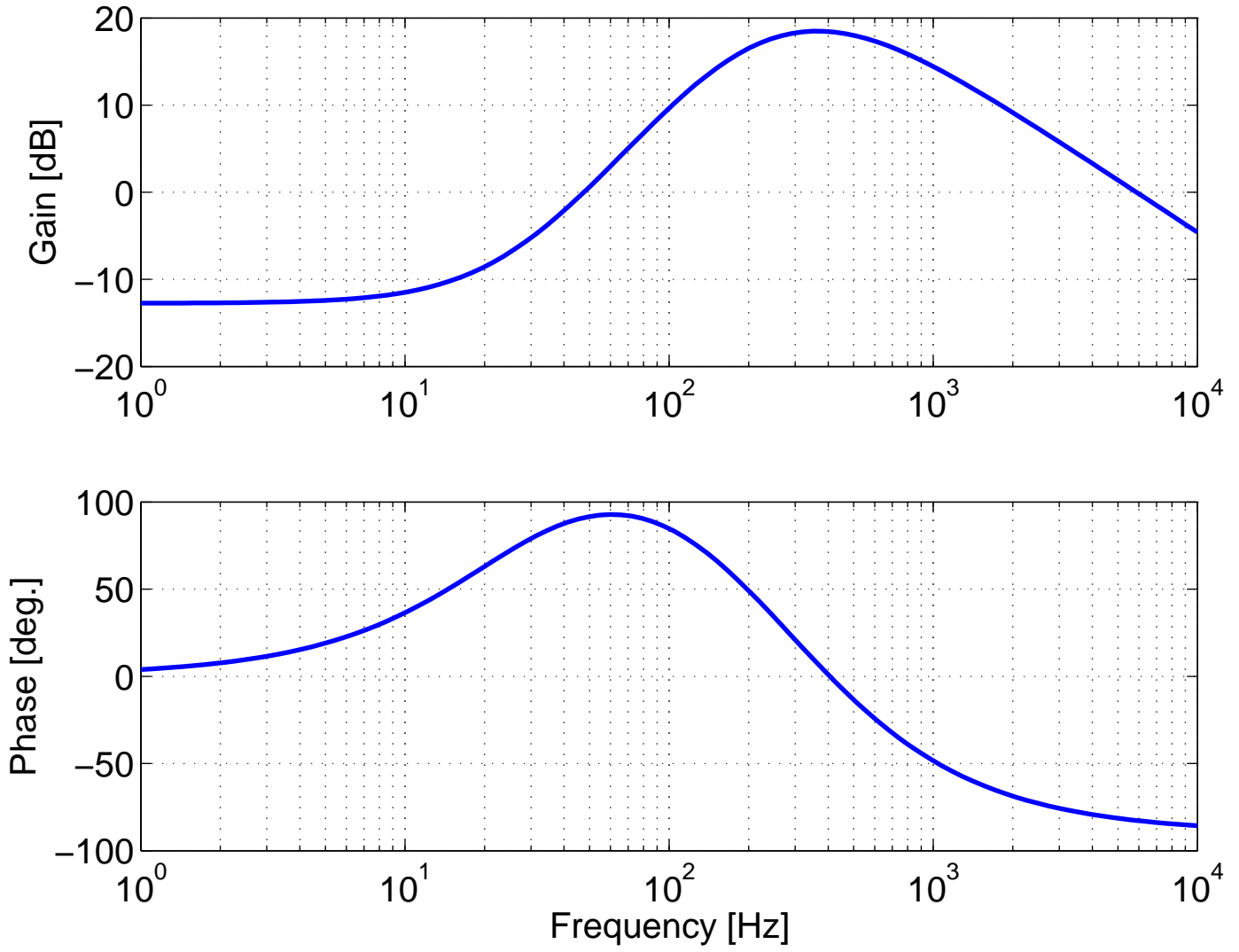
SRC Filter
