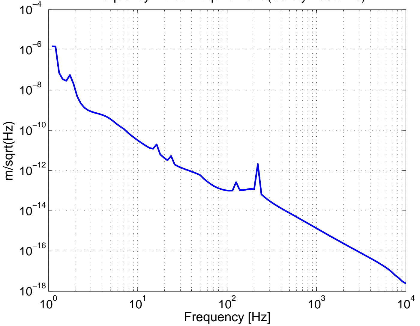
Frequency Noise Requirement (Safety Factor10)
