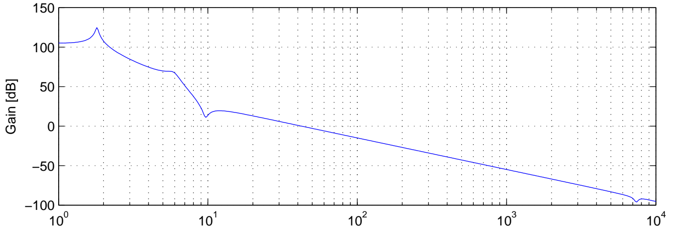
SRCL Raw Gain (without feedback filter)
