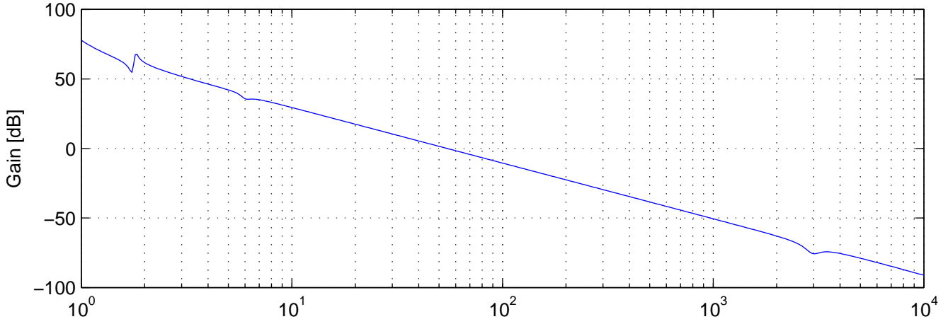
PRCL Raw Gain (without feedback filter)
