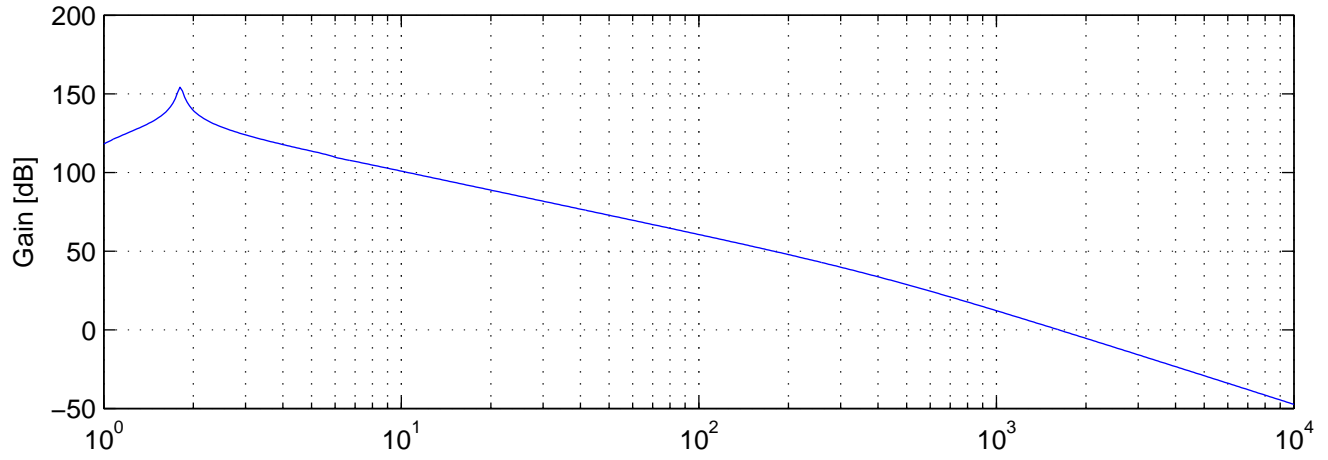
DARM Raw Gain (without feedback filter)
