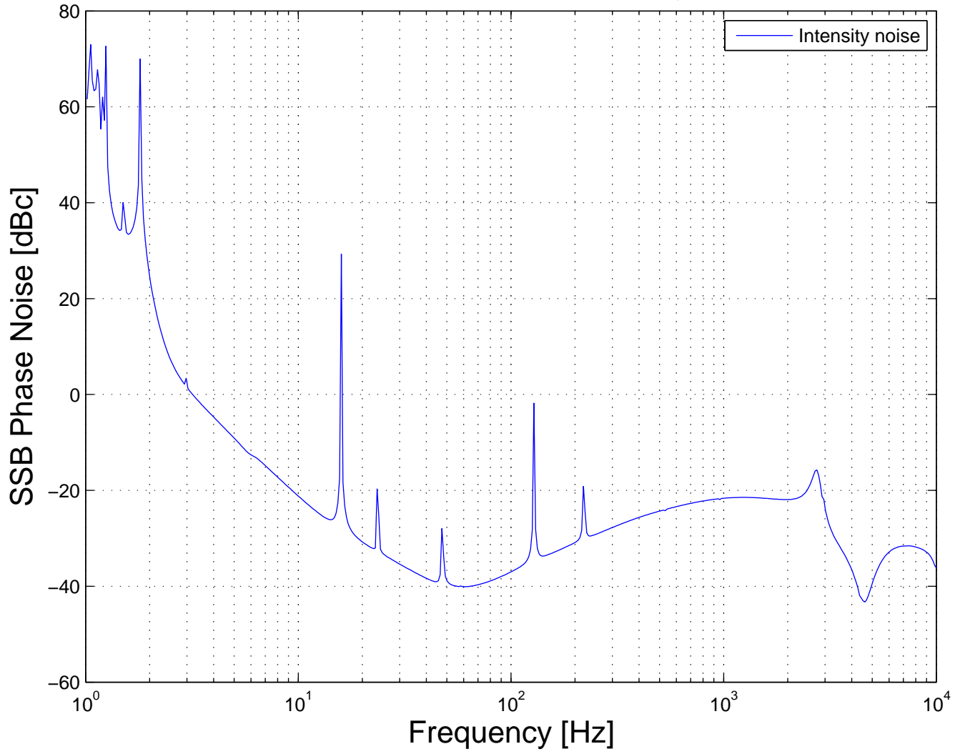
f2 SSB Phase Noise Requirement (Safety Factor 20 dBc)
