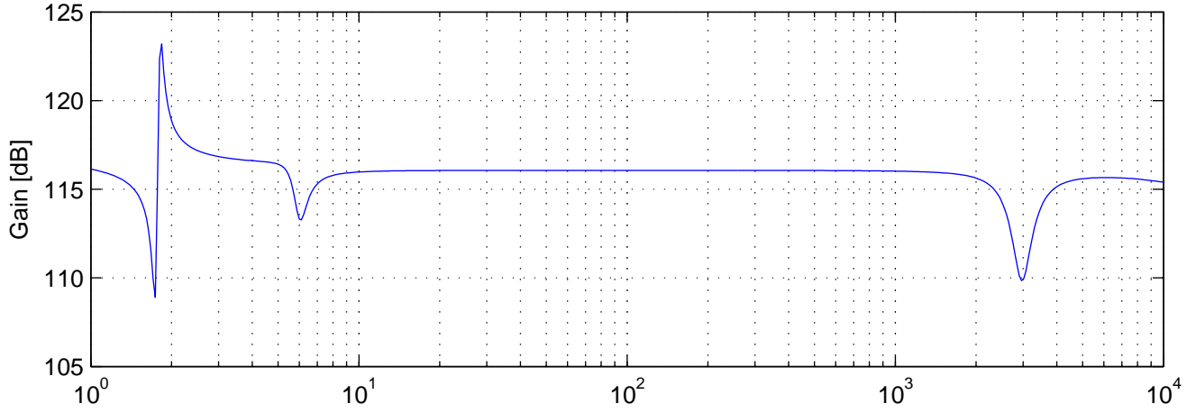
PRCL Optical Gain
