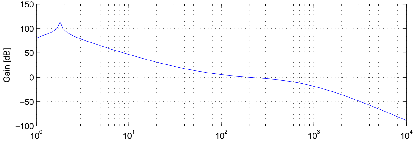
DARM Open Loop Gain
