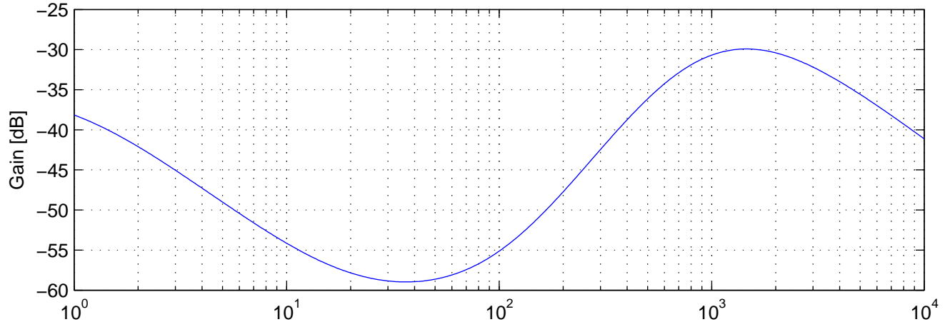
DARM Filter
