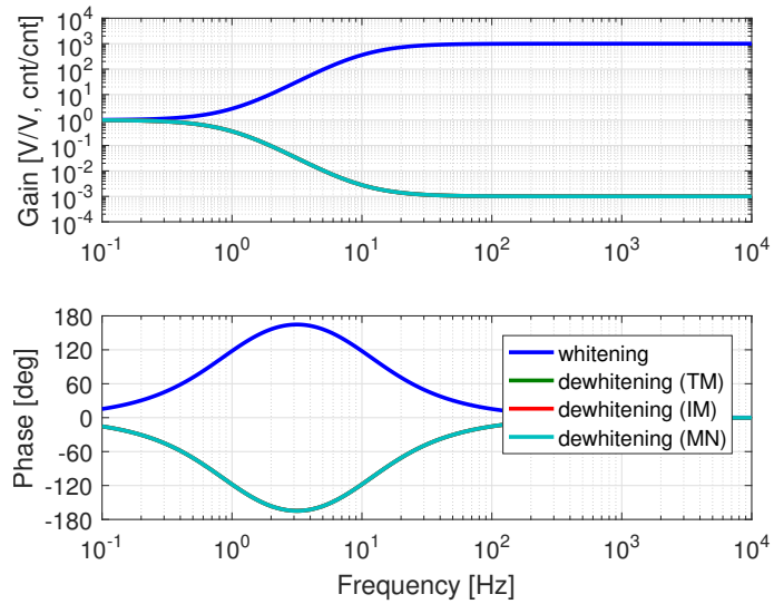
Figure 7: Whitening and dewhitening filters for IM and TM.
