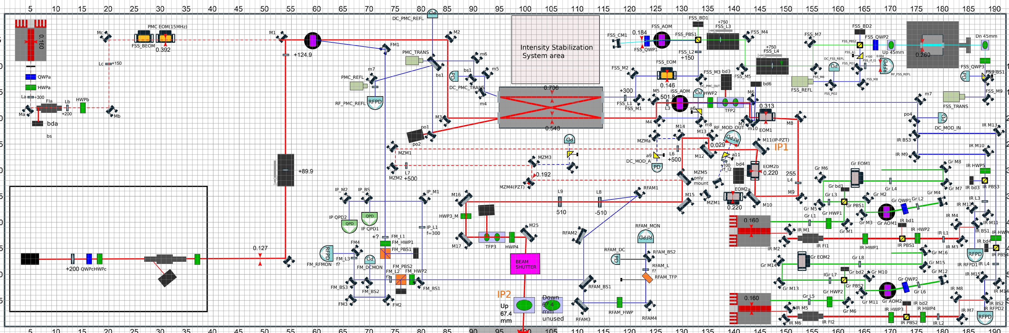
bKAGRA Input Optics Table Layout v11
