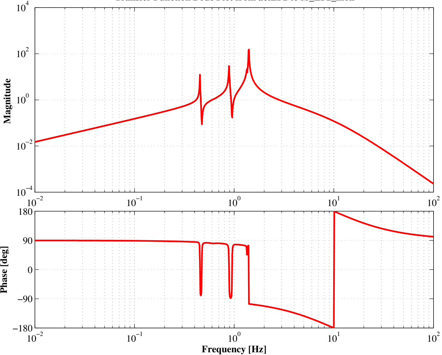
Transfer Function Bode Plot from actLF2 to fb_LF2_mon
