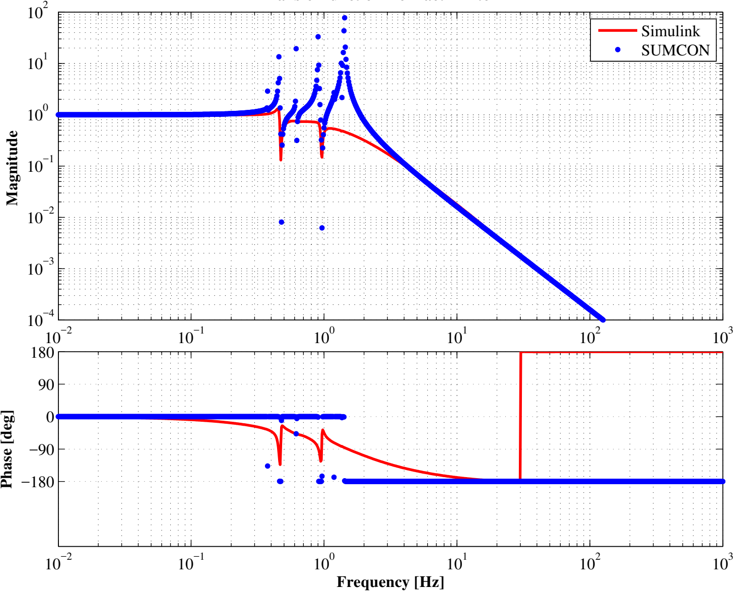
Transfer function from actTF2 to TF2
