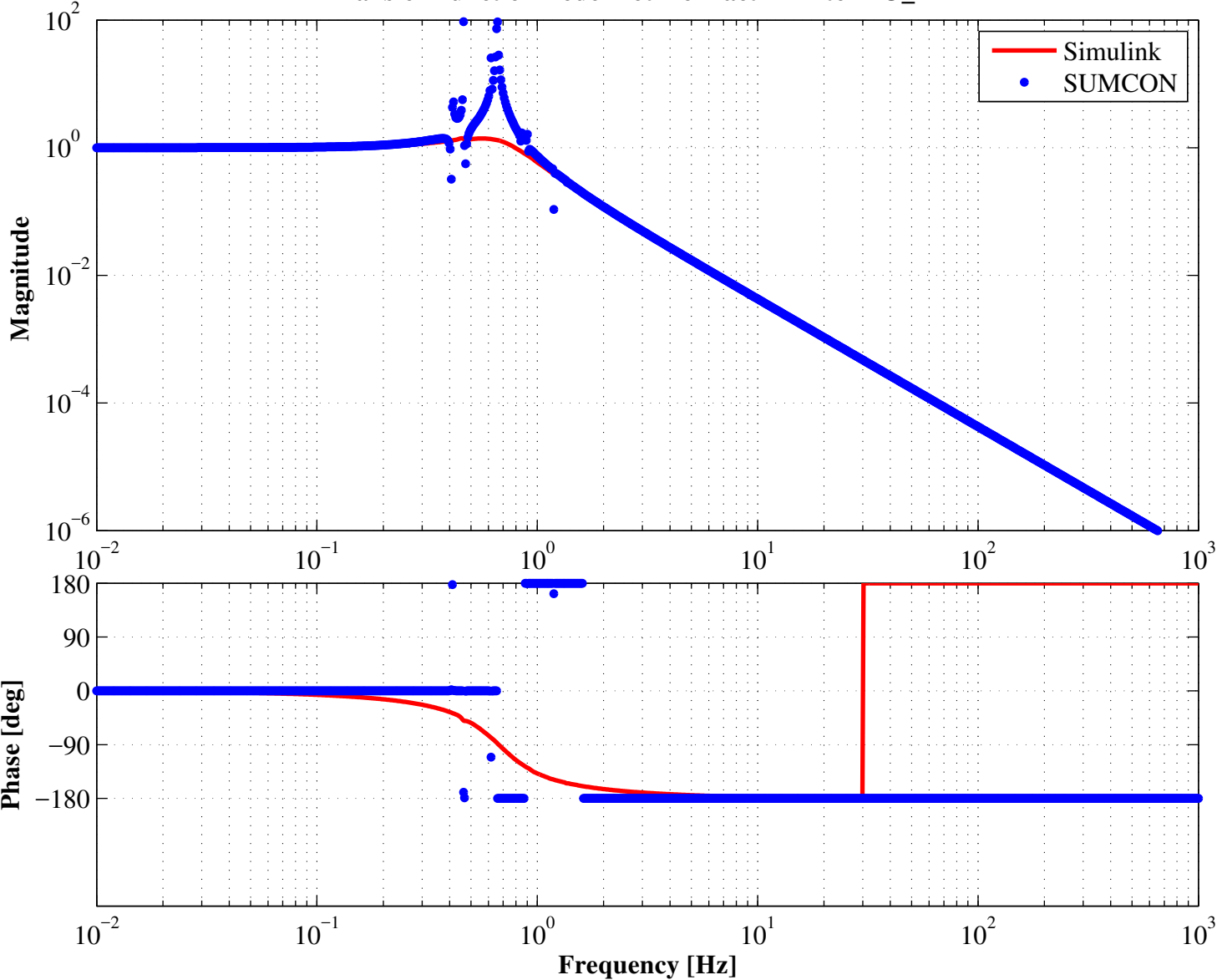
Transfer Function Bode Plot from actLTM to IFO_LTM
