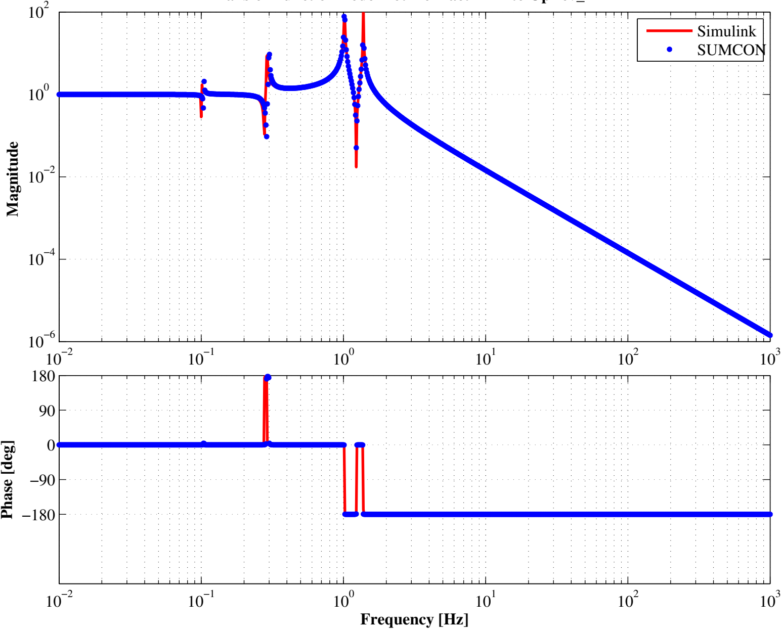
Transfer Function Bode Plot from actYTM to OpLev_YTM
