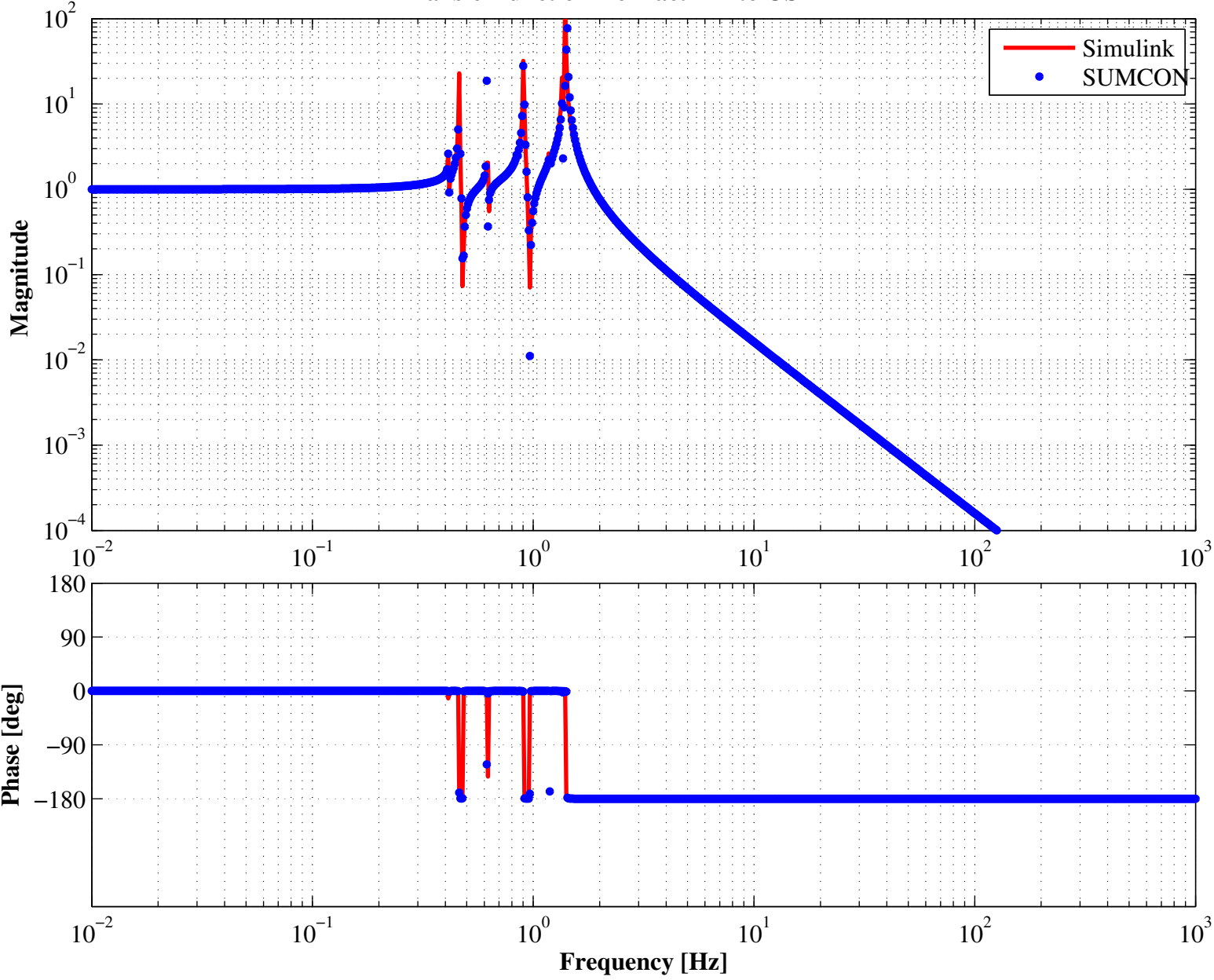
Transfer function from actLF2 to OSEM LF2
