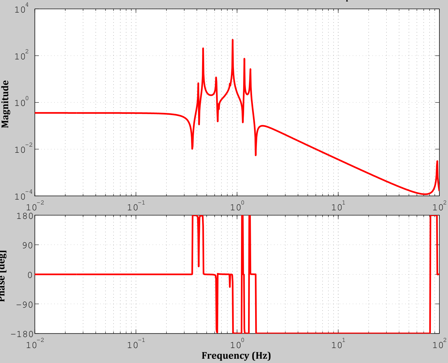
Transfer Function Bode Plot from actLF2 to OSEM p F2
