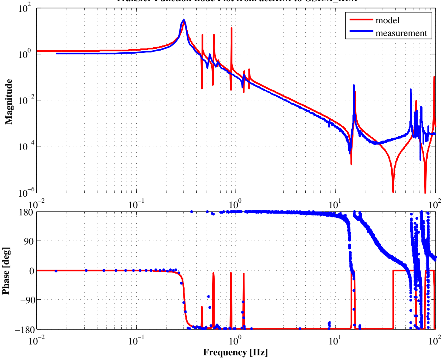
Transfer Function Bode Plot from actRIM to OSEM_RIM
