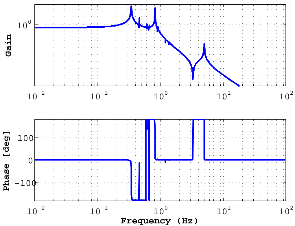
Transfer Function Bode Plot from actPIM to OplevPTM
