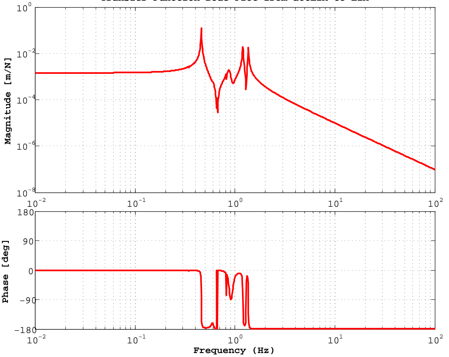
Transfer Function Bode Plot from actLIM to LIM
