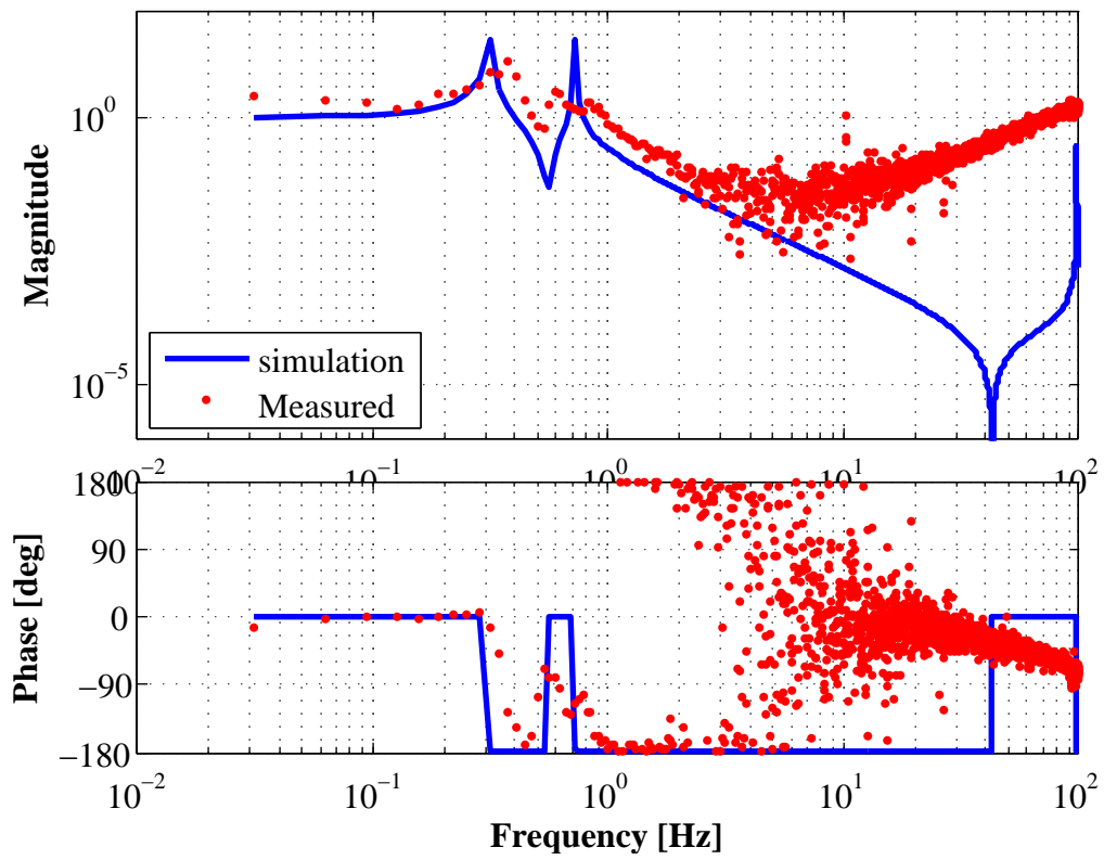
Transfer Function from actVBF to LVDT_VBF
