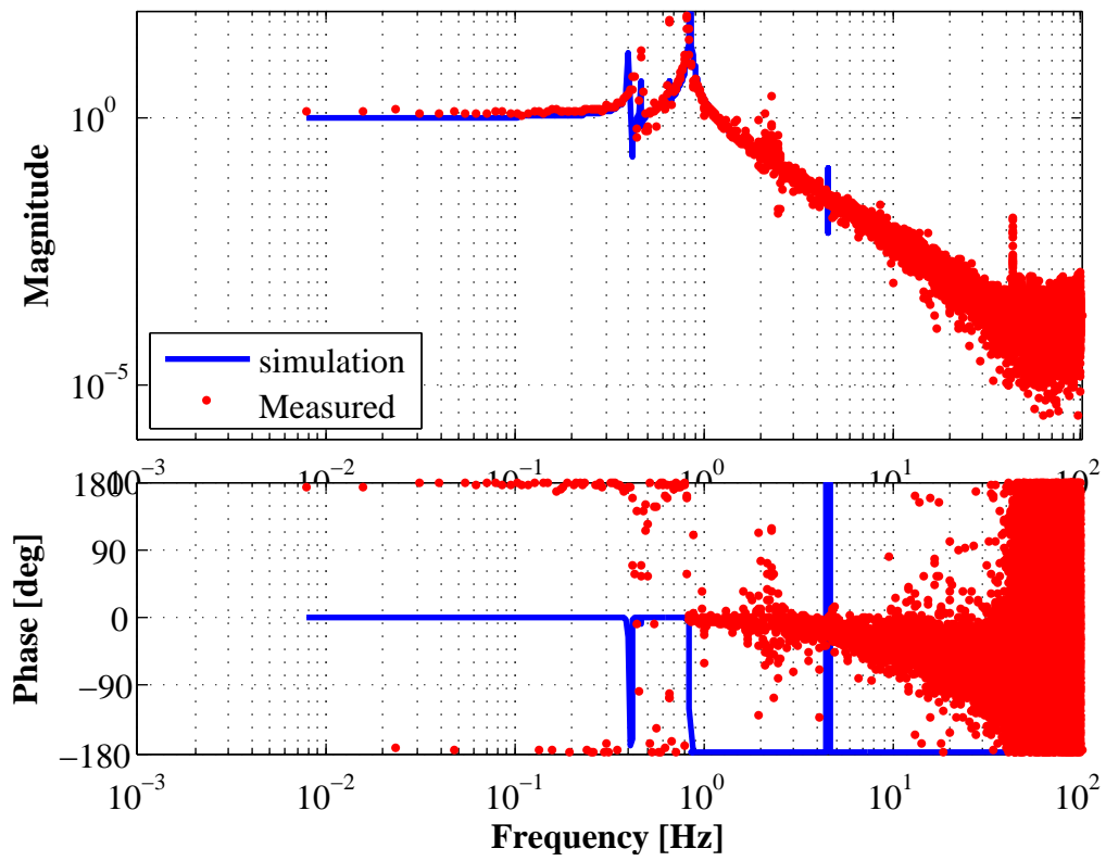
Transfer Function from actPTM to OpLev_PTM
