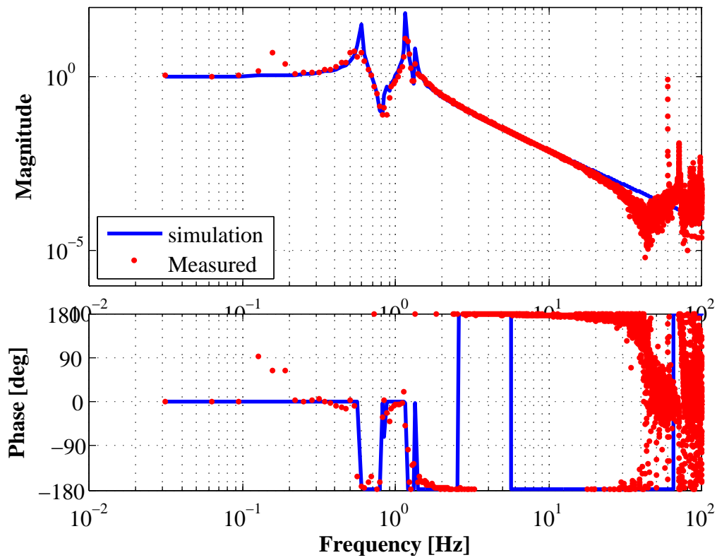
Transfer Function from actLIM to OSEM_LIM
