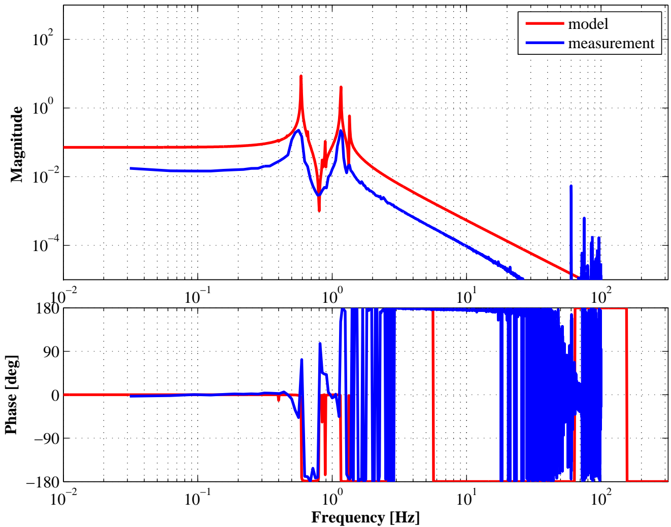
Transfer function from LIM actuator to LIM sensor
