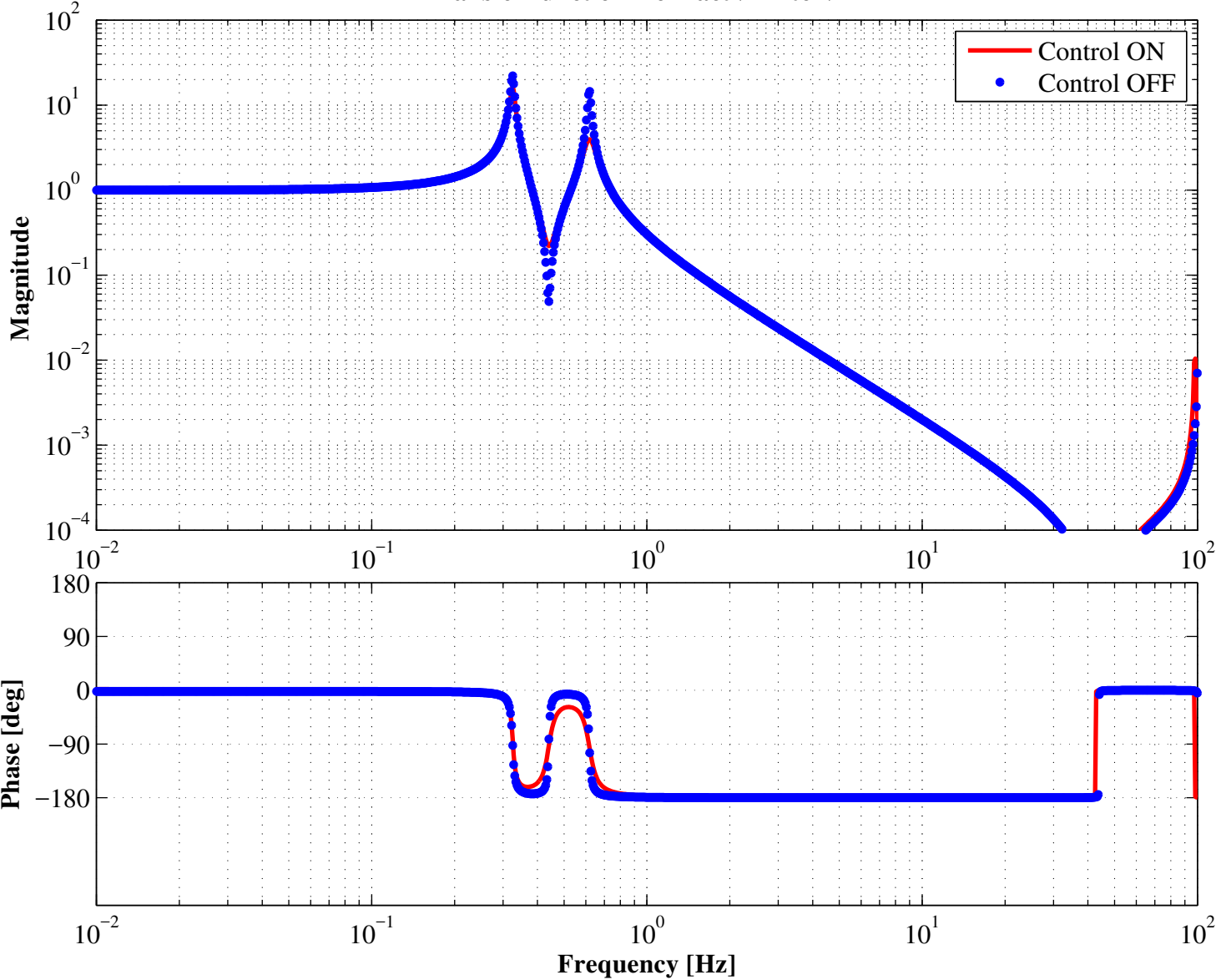
Transfer function from actVBF to VBF
