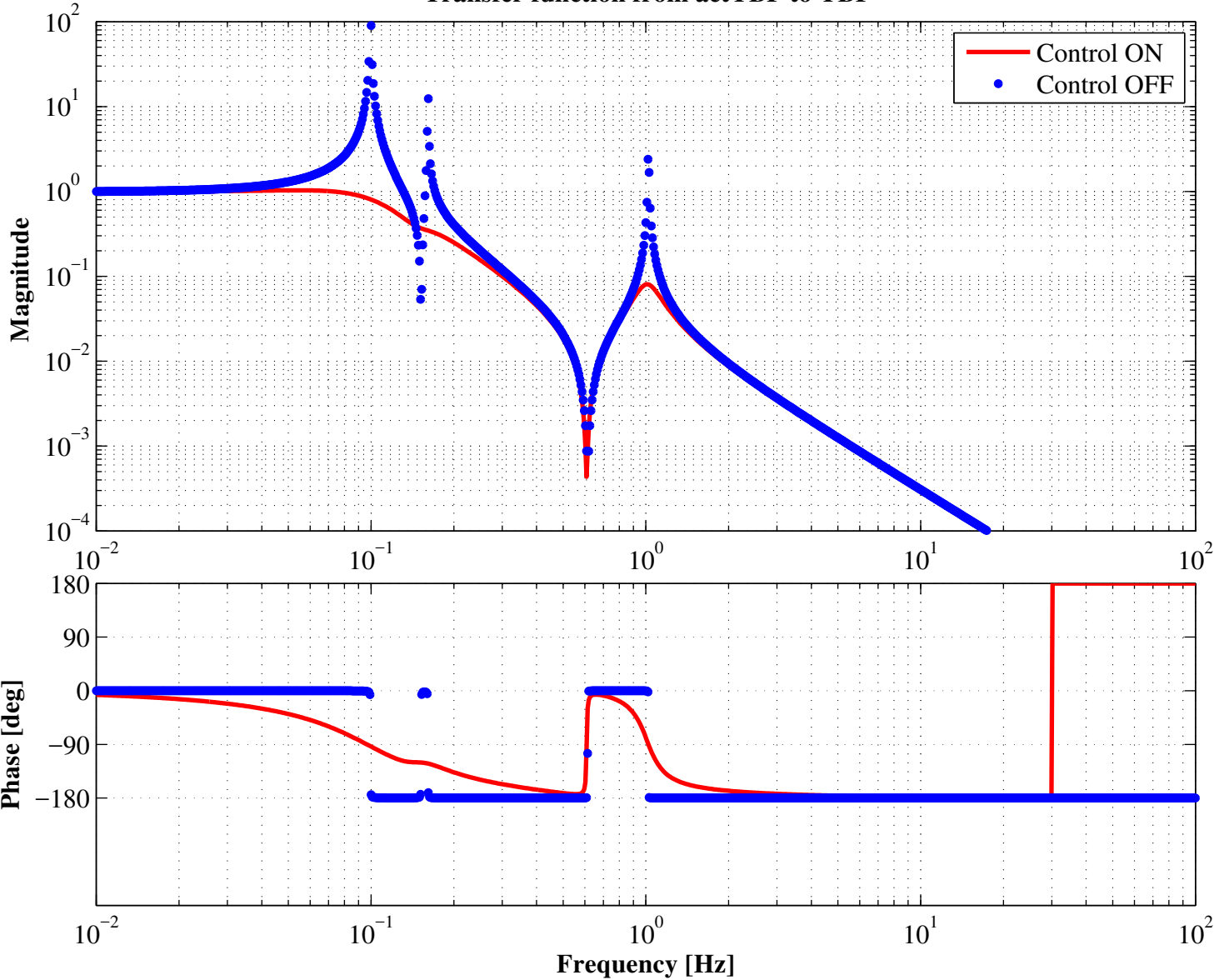
Transfer function from actYBF to YBF
