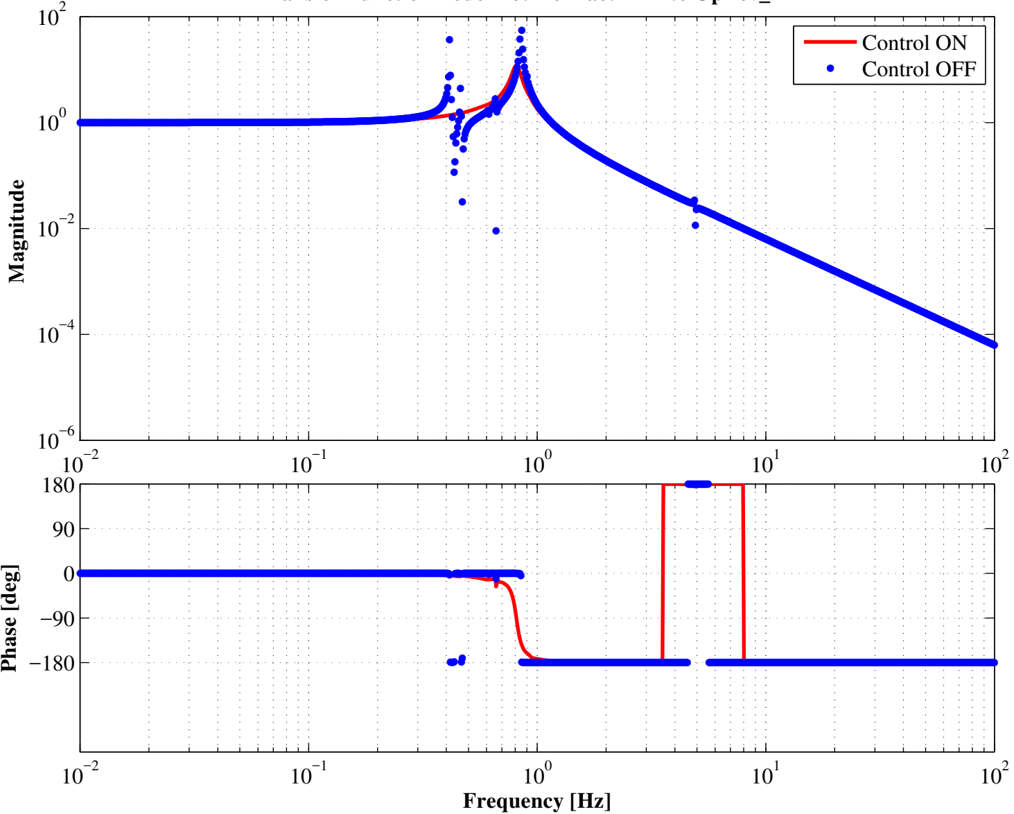
Transfer Function Bode Plot from actPTM to OpLev_PTMs
