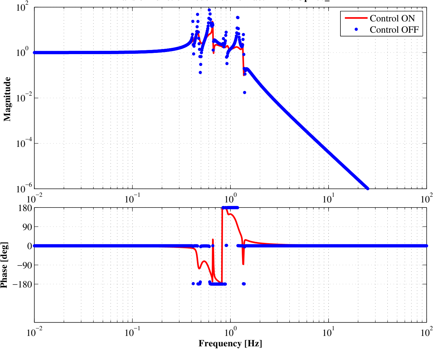
Transfer Function Bode Plot from actLIM to OpLev_LTM
