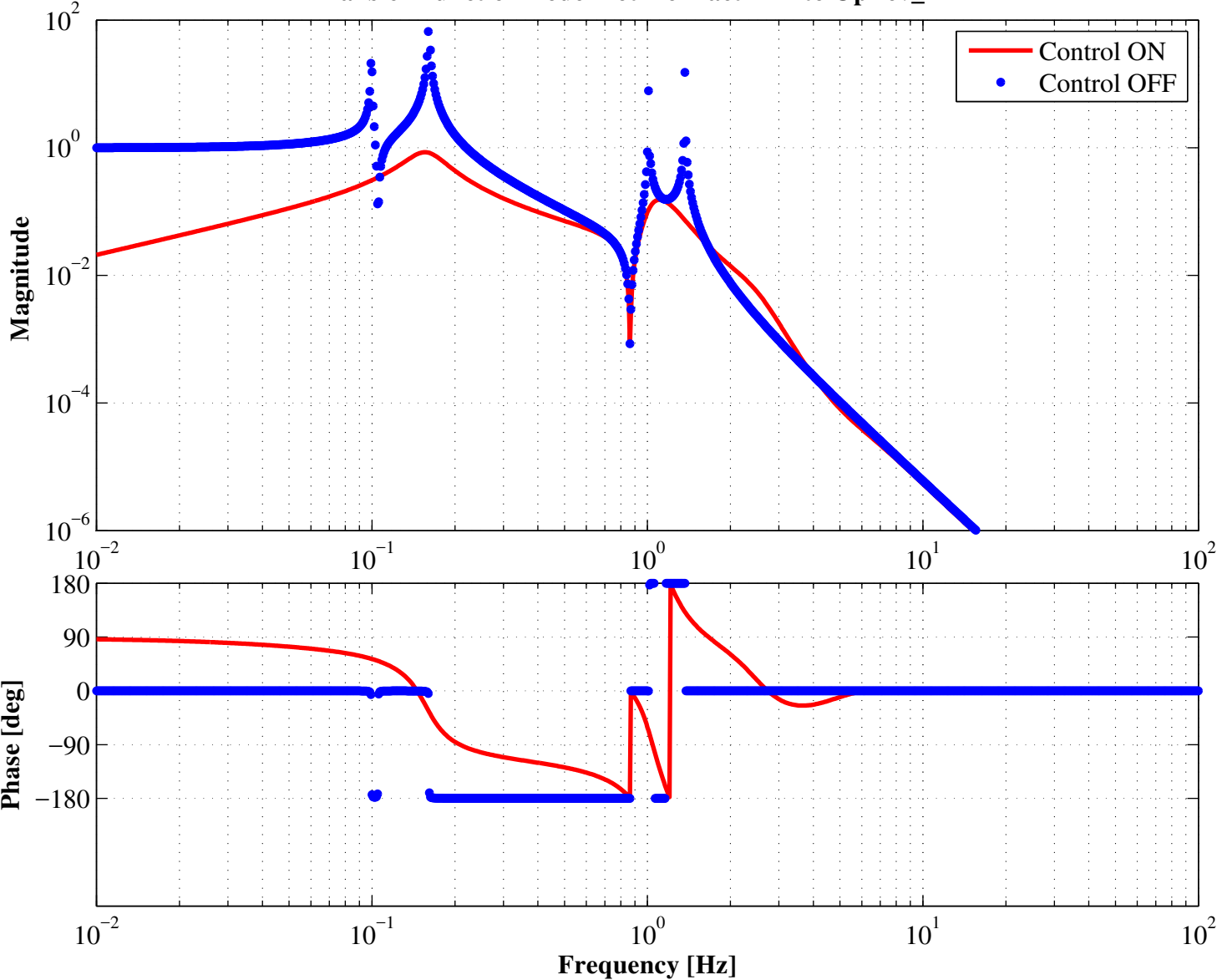
Transfer Function Bode Plot from actYIM to OpLev_YTM
