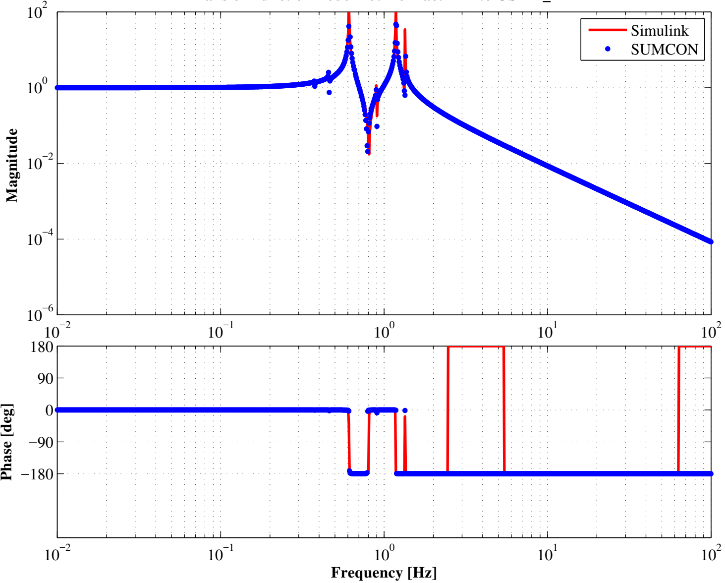
Transfer Function Bode Plot from actTIM to OSEM_TIM
