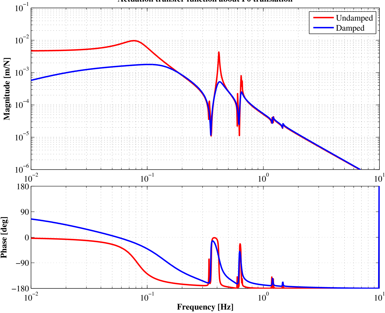
Actuation transfer function about F0 translation
