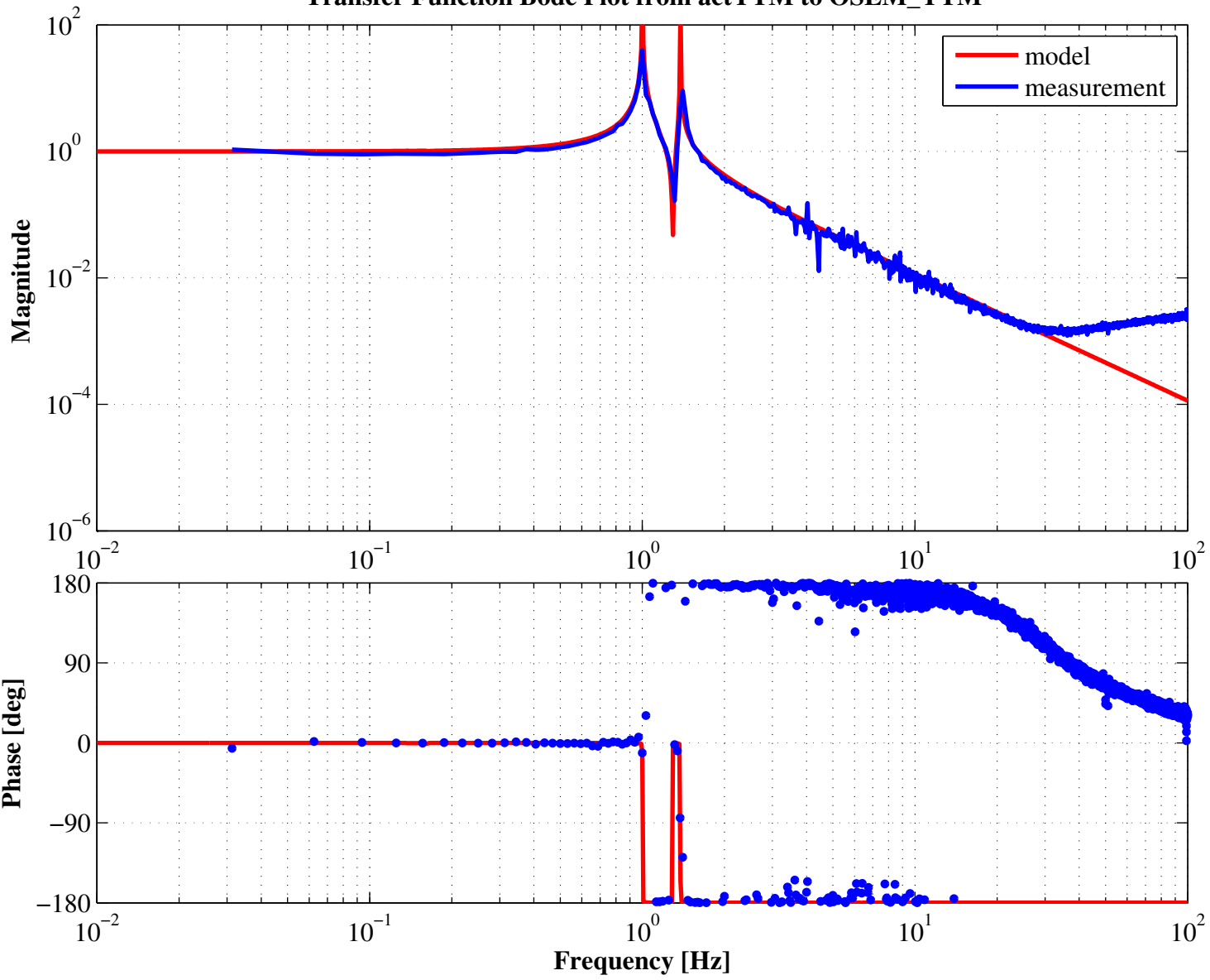
Transfer Function Bode Plot from actYTM to OSEM_YTM
