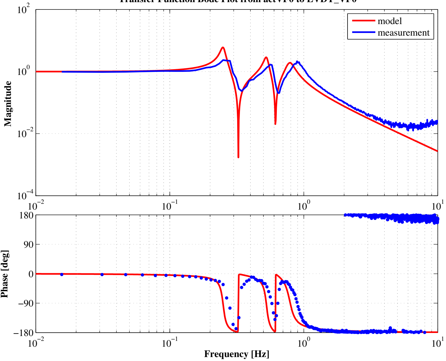
Transfer Function Bode Plot from actVF0 to LVDT_VF0
