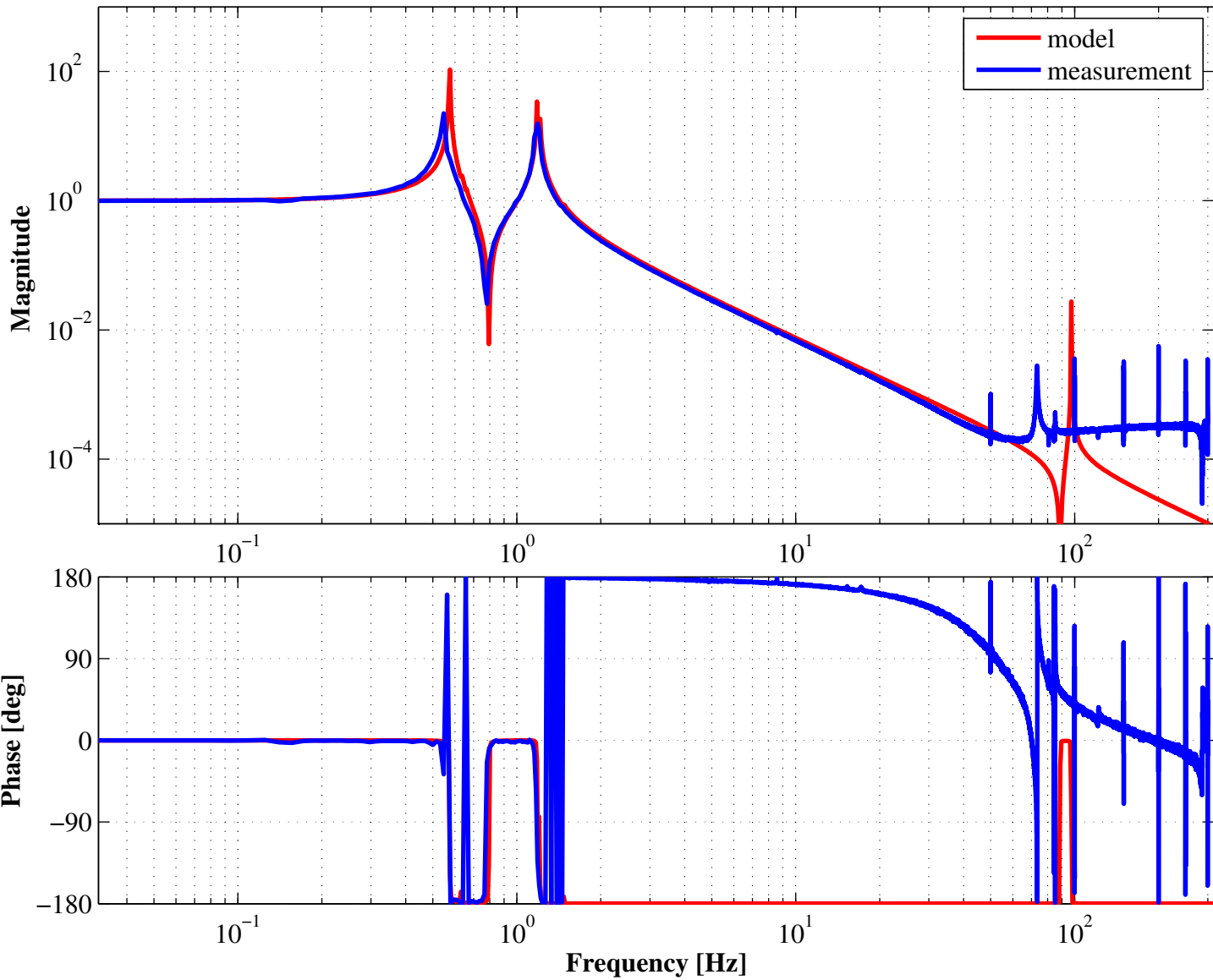
Transfer function from TIM actuator to TIM sensor
