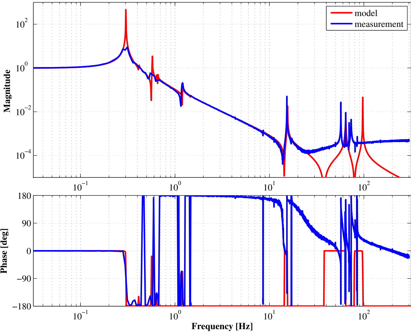
Transfer function from RIM actuator to RIM sensor
