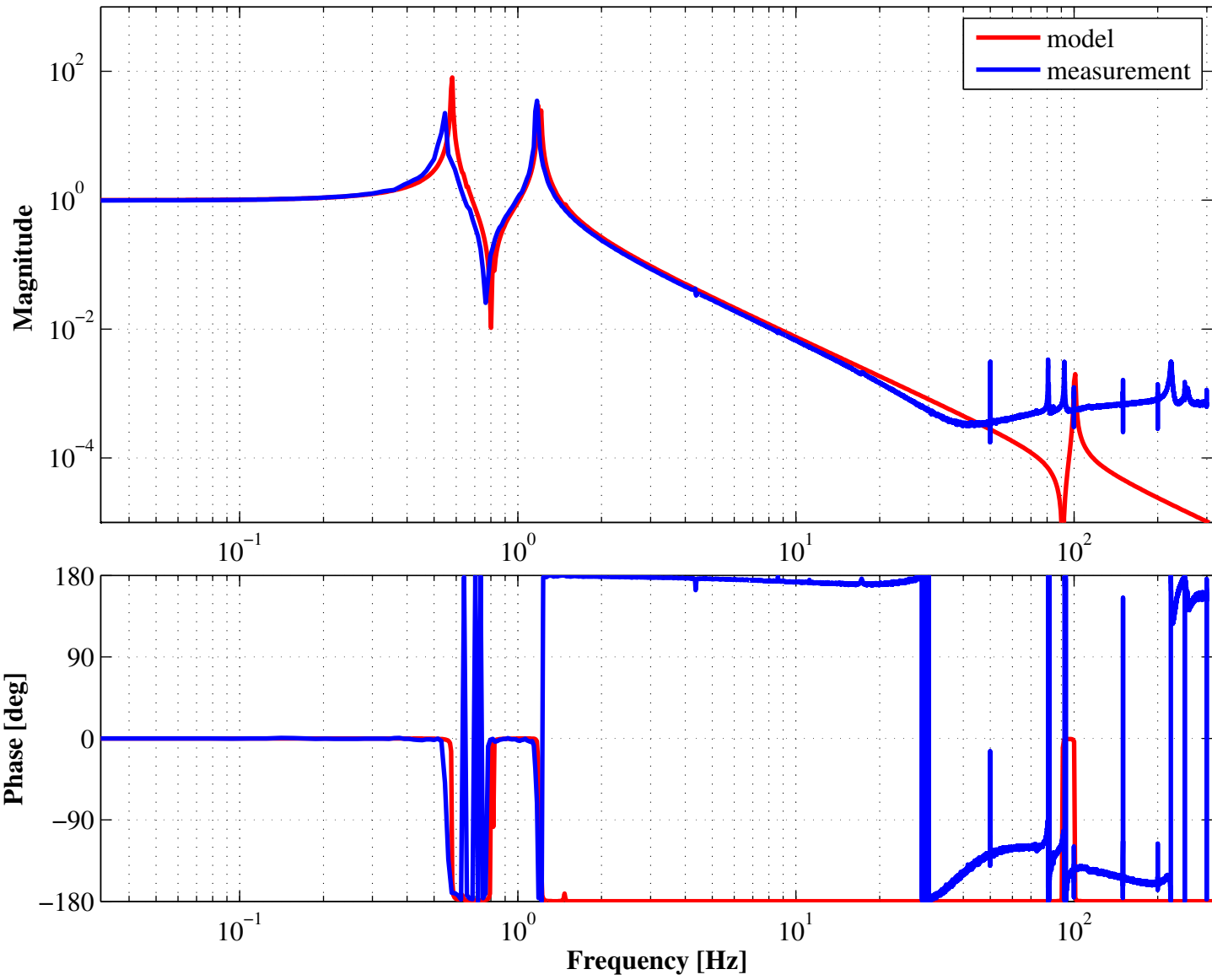
Transfer function from LIM actuator to LIM sensor
