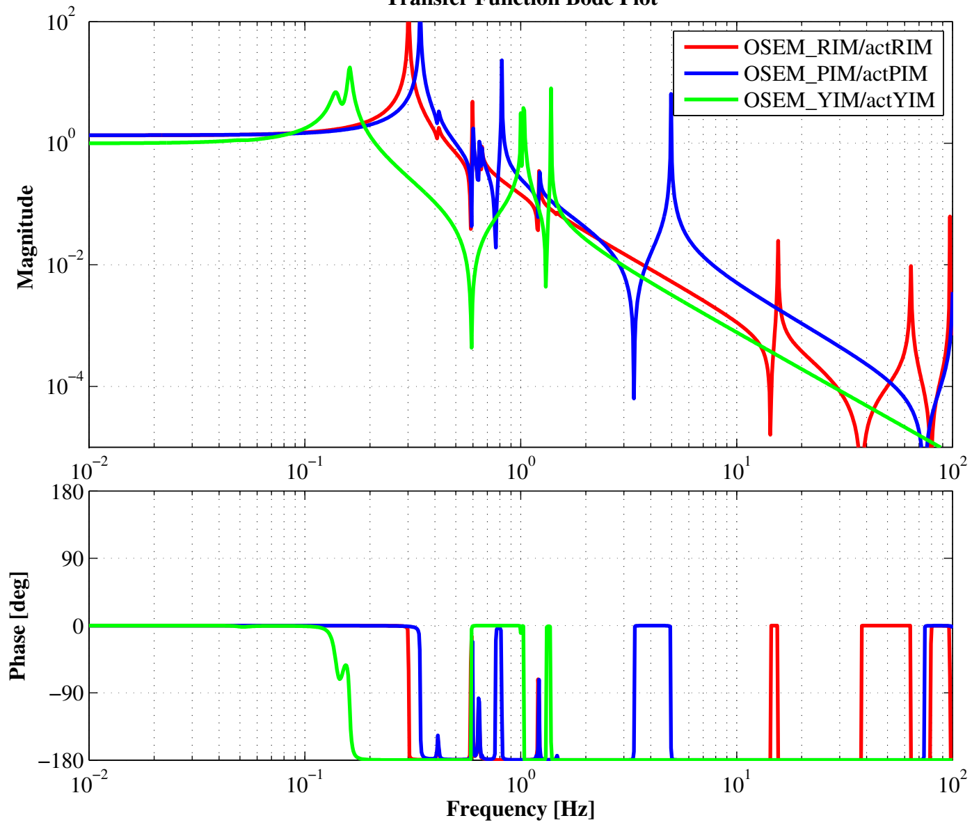
Transfer Function Bode Plot
