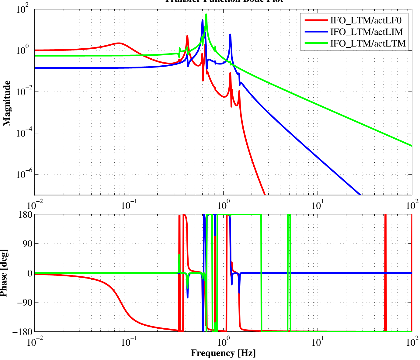
Transfer Function Bode Plot
